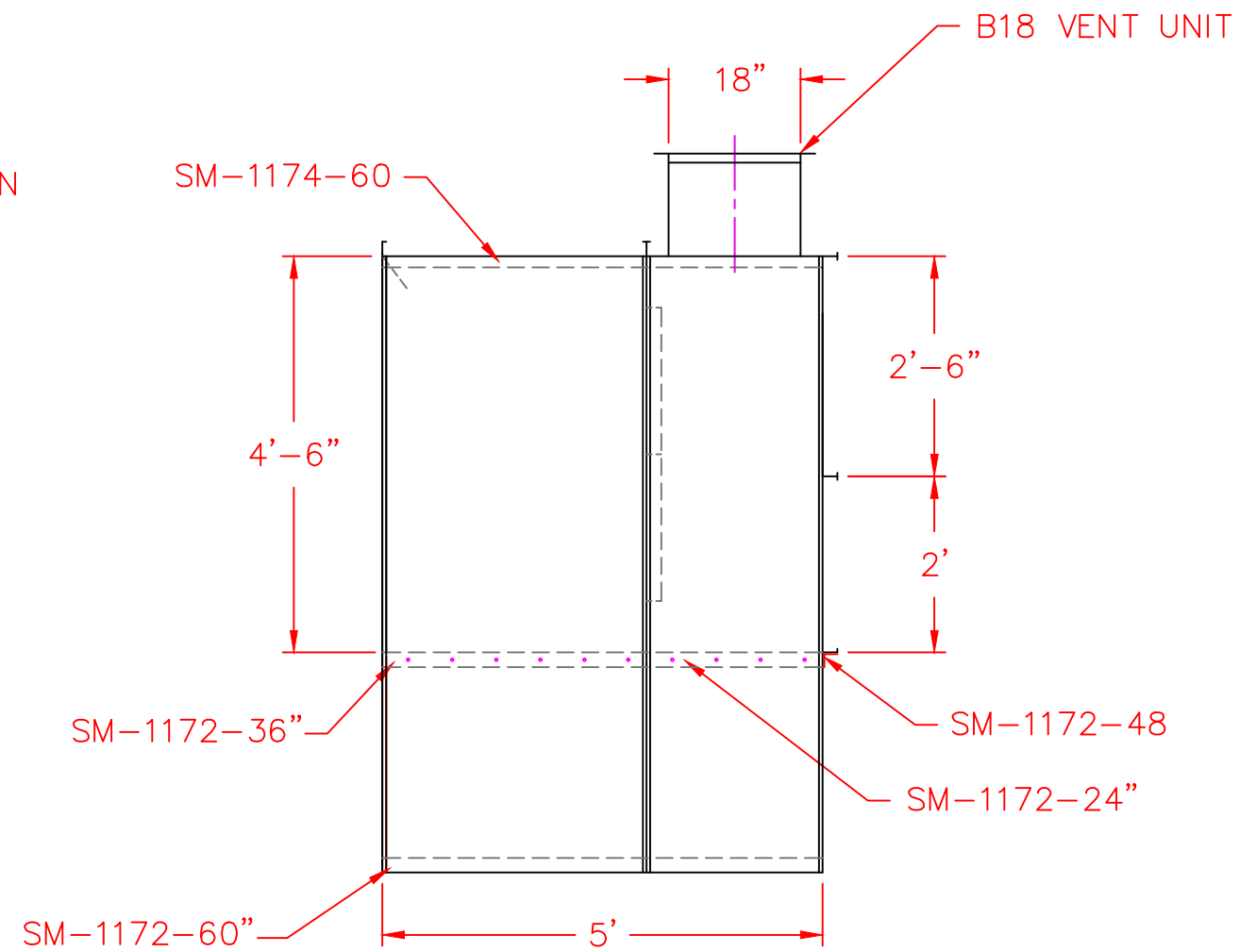
SIDE VIEW
